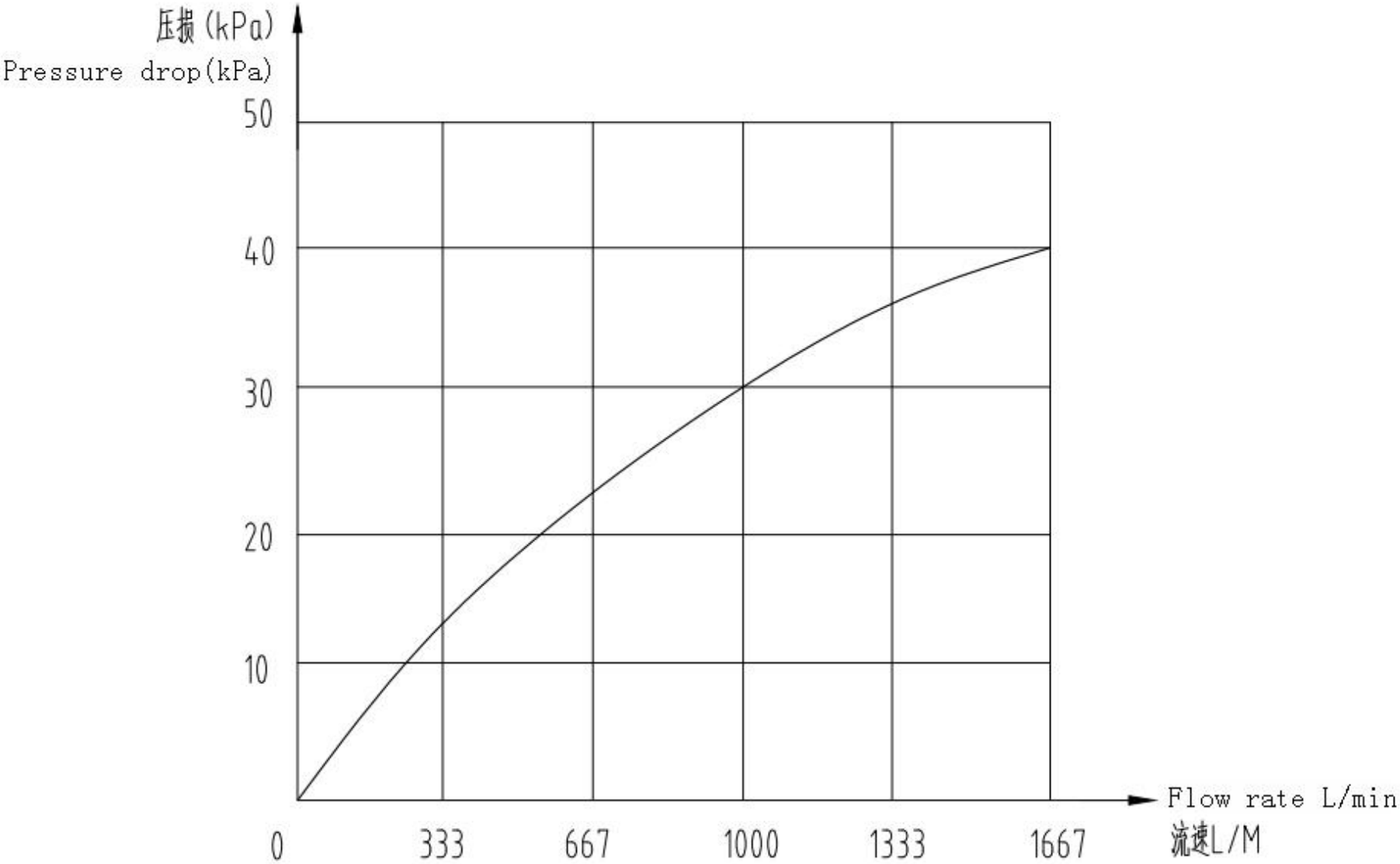
LPGX-100 (DN100)
